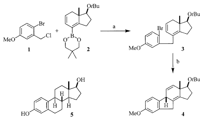
Scheme 1. (a) 5 mol % [Pd(PPh 3 ) 4 ], NaOH, THF, reflux, 22 h, 72%; (b) 5 mol % 14 , n Bu 4 NOAc, DMF/MeCN/H 2 O, 140 °C (microwave), 5 min, 70%
