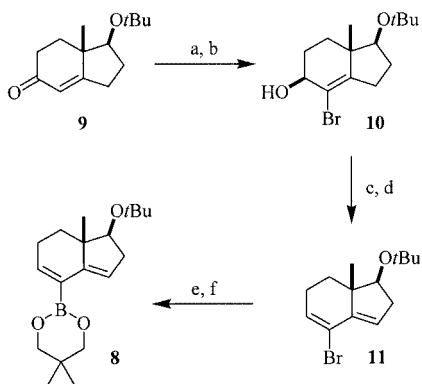
Scheme 3. (a) Br 2 , 2,4,6-collidine, Et 2 O, HOAc, room temp., dark, 24 h, 80%; (b) NaBH 4 , CeCl 3 ·7H 2 O, MeOH, room temp., 4 h, 80%; (c) MsCl, NEt 3 , CH 2 Cl 2 , room temp., 6 h; (d) DBU, 100 °C, 69% (over two steps); (e) t BuLi, TMEDA, B(O i Pr) 3 , THF, –78 °C to room temp., 1 h; (f) 2,2-dimethylpropane-1,3-diol, toluene, room temp., 16 h, 68% (over two steps)
