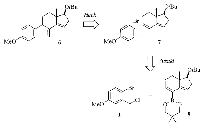
Scheme 2. Retrosynthesis of 6
