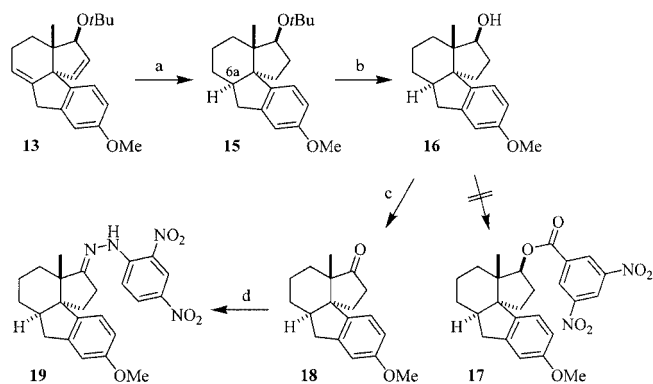
Scheme 6. (a) 20 mol % \text{PtO}_2 \cdot \text{H}_2\text{O} , \text{H}_2 , MeOH, room temp., 18 h, 96%; (b) TMSI, \text{CH}_2\text{Cl}_2 , room temp., dark, 16 h, 97%; (c) DMP, \text{CH}_2\text{Cl}_2 , room temp., 6 h, 76%; (d) 2,4-dinitrophenylhydrazine, \text{H}_2\text{SO}_4 , EtOH, room temp., 1 h, 77%
