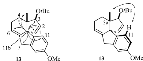
Scheme 5. Structure determination of 13 by HMBC and NOE experiments
