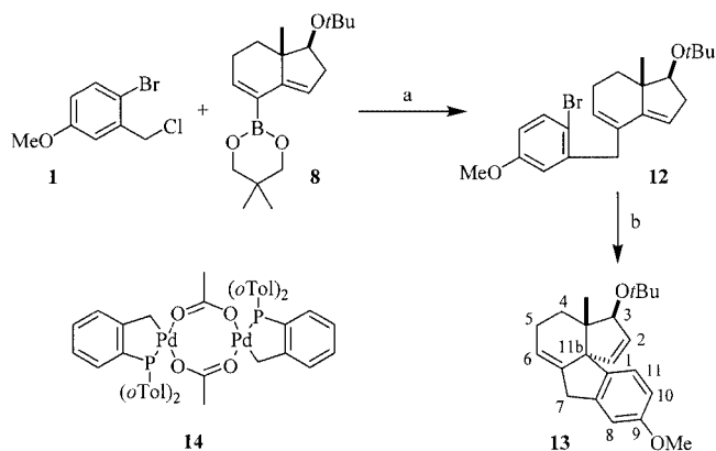
Scheme 4. (a) 5 mol % [Pd(PPh 3 ) 4 ], NaOH, THF, reflux, 16 h, 77%; (b) 5 mol % 14 , n Bu 4 NOAc, DMF/MeCN/H 2 O, 180 °C (microwave), 30 min, 73%
